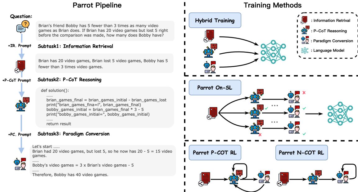
Figure 2: The training pipeline and methods of Parrot . On the left, the pipeline consists of three subtasks: Information Retrieval , P-CoT Reasoning , and Paradigm Conversion . By these subtasks, the model sequentially generates P-CoT and n-CoT. On the right, we use a Hybrid Supervised Fine-Tuning (SFT) strategy to enable semantic transfer and incorporate reinforced algorithms for further improvements. The detailed Parrot inference process and subtask prompts are provided in Appendix A.3.
