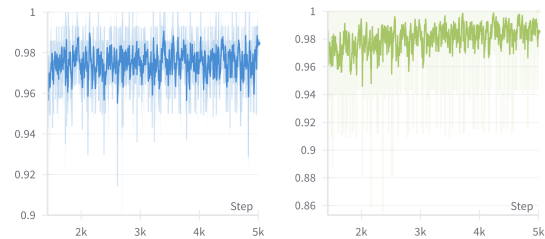
Figure 3: The training accuracy of LLaMA-2-7B on SVAMP for P-CoT RL. The left figure is without the converted penalty while the right is with the penalty.
