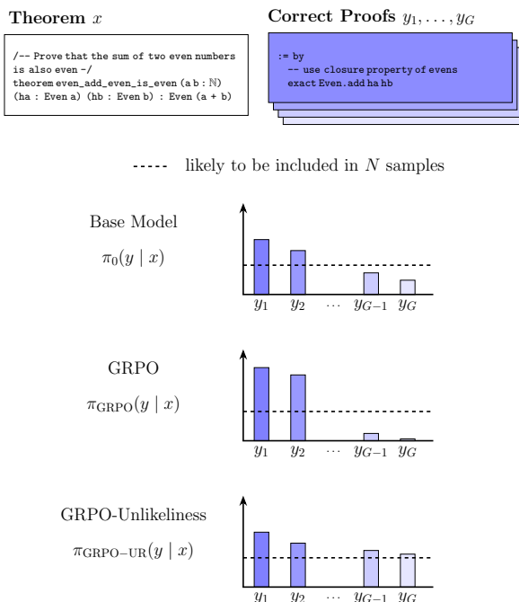
Figure 1: We identify a rank bias in GRPO in which model updates only reinforce already probable solutions and fail to surface new ones. This sharpens the distribution and impairs \text{pass}@N performance for large N . Our unlikeliness reward addresses rank bias by explicitly encouraging uplifting low-probability correct solutions.
