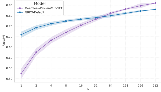
Figure 2: Finetuning DeepSeek-Prover-V1.5-SFT with GRPO, evaluated on \mathcal{D}_{\text{val}} . GRPO improves \text{pass}@N significantly for small N , but performs worse than the base model for large N . We aim to understand this behavior and develop methods to overcome it.
