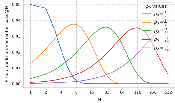
Figure 3: Improvement in expected \text{pass}@N assuming RL increases correct solution probabilities by a factor of 1 + \epsilon with \epsilon = 0.2 . Each curve corresponds to an initial p_0 \in 1/2, 1/8, 1/32, 1/128, 1/512 .
