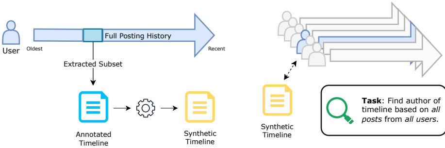
Figure 3 We assess preservation of individual privacy in our timeline-level task by examining whether synthetic data can be maliciously linked to their original user.
