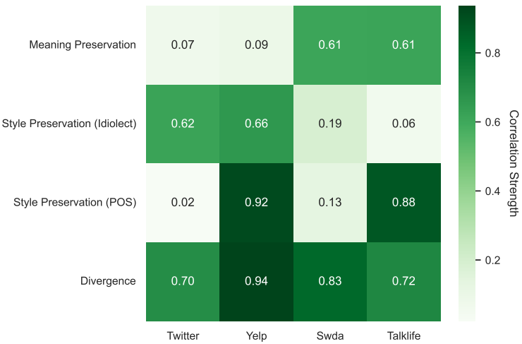
Figure 5 Absolute Spearman’s rank correlation between sample-level and distribution-level metric values.
