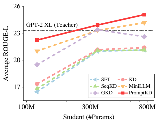
Figure 1: Comparison of instruction-following performance of KD methods using the GPT-2 model family. Owing to the student-friendly knowledge, our PromptKD outperforms others with only an additional 11K parameters. Dashed reference line represents the performance of the teacher model.
