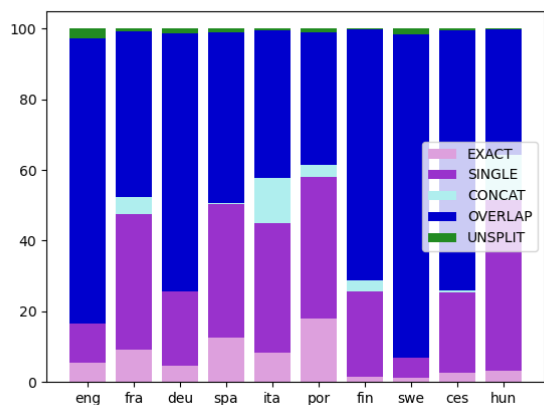
Figure 1: Segmentation categories per language.
