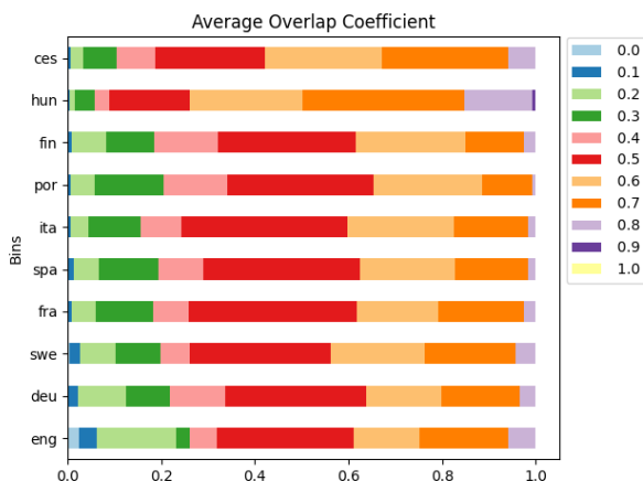
Figure 2: Distribution of overlap scores per inflection paradigm for verbs. The scores are rounded to the nearest decimal, resulting in ranges of 0.1
