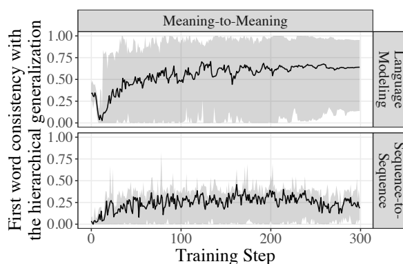
Figure 6: First word consistency with the hierarchical generalization for models trained on the MEANING TO MEANING dataset. The black line indicates the average across 10 random reruns. Light gray shaded areas are the minimum and maximum values for any model at each training step across the 10 random reruns.
