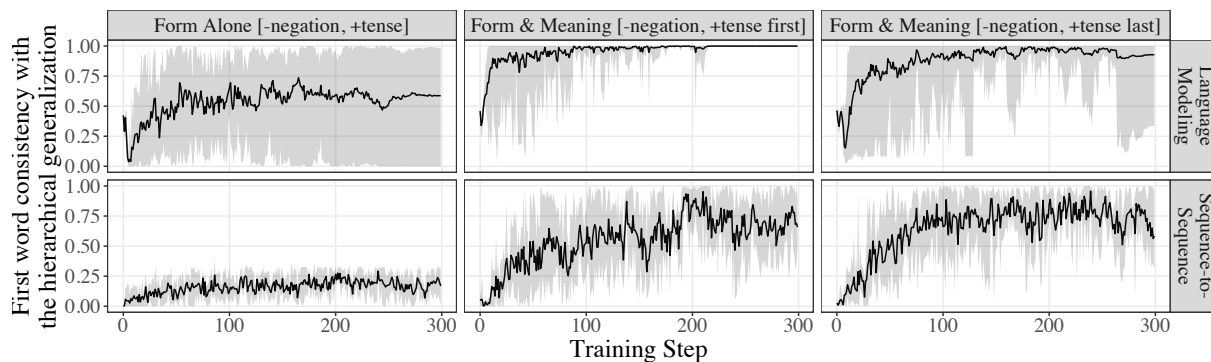
Figure 5: First word consistency with the hierarchical generalization for models trained on the [+tense] datasets. Top: models trained in a language modeling setup. Bottom: models trained in a sequence-to-sequence setup. The black line indicates the average across 10 random reruns. Light gray shaded areas are the minimum and maximum values for any model at each training step across the 10 random reruns.
