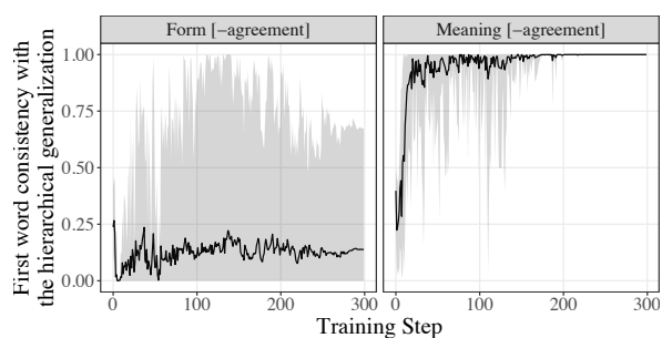
Figure 8: First word consistency with the hierarchical generalization for models trained on the [-agr] datasets. The black line indicates the average across 10 random reruns. Light gray shaded areas are the minimum and maximum values for any model at each training step across the 10 random reruns.
