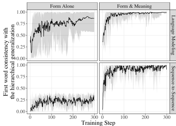
Figure 3: Left: first word accuracy across 300k training steps for models trained on FORM ALONE (left) or FORM AND MEANING (right), in a language modeling (top) or sequence-to-sequence (bottom) setup. The black line indicates the average across 10 random reruns. Light gray shaded areas are the minimum and maximum values for any model at each training step across the 10 random reruns. All models reach in-domain saturation (>99% full question accuracy) by 10k training steps.
