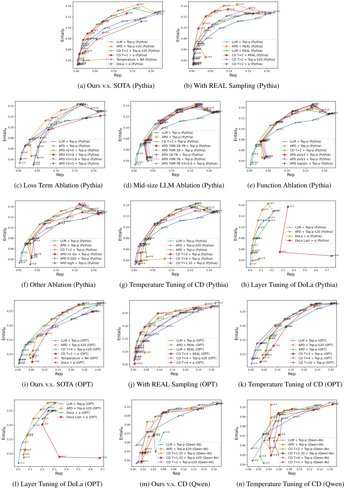
Figure 9: FACTUALITYPROMPTS results using factual prompts. The curves closer to the upper left corner are better. The average standard error of \text{Entail}_R is 0.0031 and the maximal one is 0.0095.
