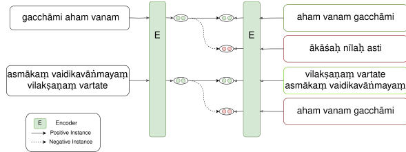
Figure 3: Schematic illustration of the proposed approach for Sanskrit. Self-supervised CSSL leverages the sentence and its permutation pairs as positives and other in-batch instances as negatives.
