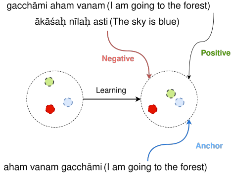
Figure 2: The Contrastive Loss minimizes the distance between an anchor (blue) and a positive (green), both of which have a similar meaning, and maximizes the distance between the anchor and a negative (red) of a different meaning.
