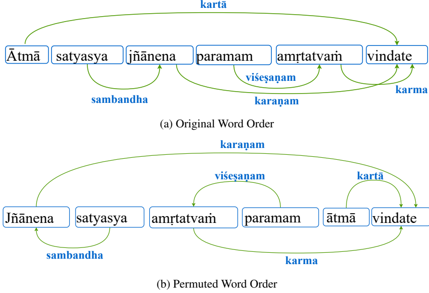
Figure 1: The Dependency Parse of a Sanskrit sentence and its random permutation is same, exhibiting free-word-order nature of the language. Translation: "The soul attains supreme immortality through the knowledge of truth."
