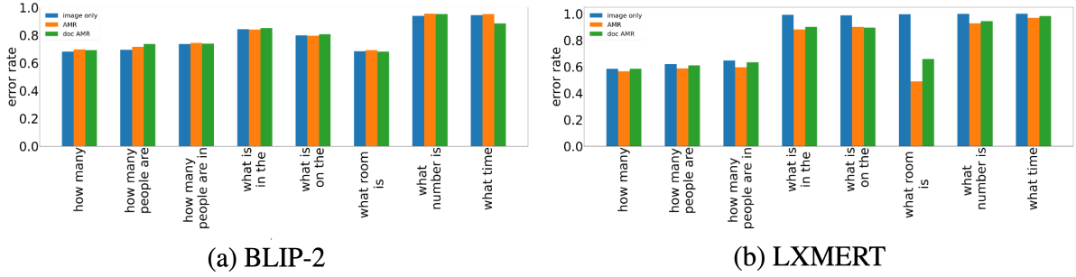
Figure 4: Error rates by question type (as listed in Table 4) for models trained in a low-resource setting (section 3). (a) shows results for BLIP-2, and (b) for LXMERT.
