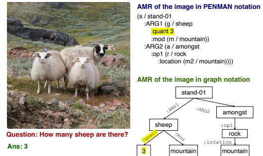
Figure 1: An example from the COCO-VQA dataset, where the AMR is generated from the longest image description available in the COCO captions. The AMR appears in PENMAN (text-based) notation (Kasper, 1989) and as a graph. Notably, the :quant node in the AMR encodes the correct answer to the question.
