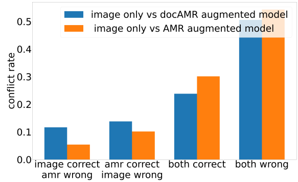
(b) LXMERT
