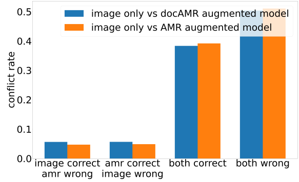
(a) BLIP-2
