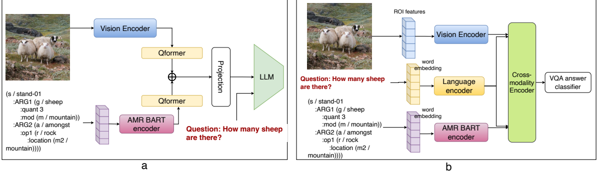
Figure 2: Updated model architectures for AMR-augmented vision-language models. (a) AMR integration in BLIP-2: a dedicated Q-former processes AMR embeddings, which are then combined with image features before being passed to the language model. (b) AMR augmentation in LXMERT: AMR embeddings from AMRBART are fed into a separate modality stream, which is later cross-attended by the language stream alongside visual features.
