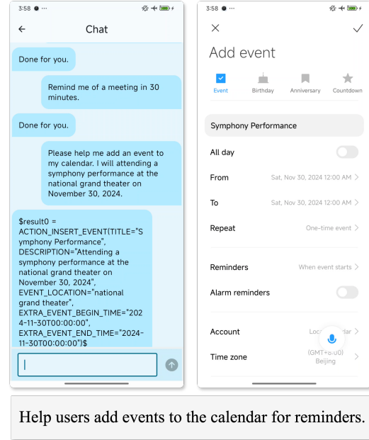
Figure 1: Small language models fine-tuned with DroidCall have the capability to assist users in completing common tasks such as adding events to the calendar.
