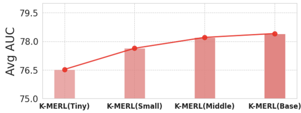
Figure 9: Reported performance of zero-shot classification with scaled ECG encoders. As the model size increases from K-MERL(Tiny) to K-MERL(Base), the performance improves, demonstrating the scalability of the model.
