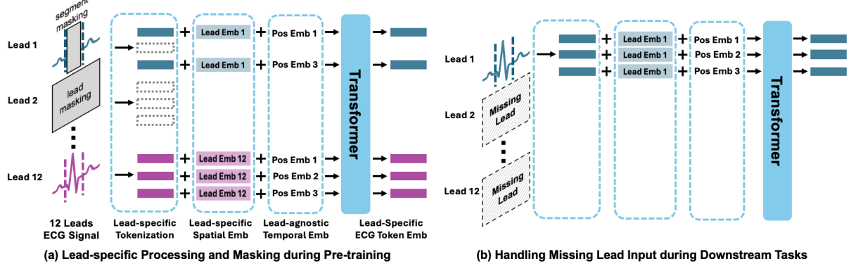
Figure 2: Illustration of our lead-specific processing and handling of partial leads input in K-MERL. (a) : Lead-specific processing and masking during pre-training. The model employs lead-specific tokenization, spatial embeddings, and lead-agnostic temporal embeddings to capture spatial-temporal patterns for each lead (see Sec 2.2). Dynamic lead masking is used to simulate inputs with arbitrary combinations of leads, while segment masking encourages the framework to capture temporal patterns (see Sec 2.3). (b) : Handling partial lead input during downstream tasks. When leads are missing, the model processes only the available leads using lead-specific embeddings, allowing maintained performance even with incomplete data.
