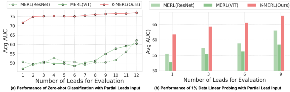
Figure 6: Performance of Zero-shot Classification with Partial Leads Input. (a) Zero-shot classification shows K-MERL consistently outperforming MERL with two backbones across all lead combinations from 1 to 12. (b) Linear probing with 1% data demonstrates K-MERL’s superior performance and robustness, even with limited data and varying lead inputs.
