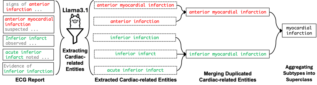
Figure 3: Illustration of mining structured knowledge from free-text reports (see Sec 2.4). First, cardiac-related entities are extracted from free-text ECG reports using an open-source LLM (e.g., Llama3.1-70B-Instruct). Next, we query the LLM to merge duplicated or synonymous cardiac-related entities into a list of unique names. Finally, the LLM detects and aggregates subtypes into their respective superclasses, creating a structured hierarchy of cardiac-related entities.
