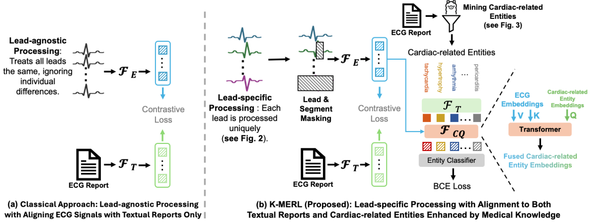
Figure 1: Comparison between classical ECG multimodal learning and our K-MERL framework. (a) : The classical approaches (e.g., MERL (Liu et al., 2024)) are suboptimal: they process all leads in a lead-agnostic manner and naively align ECG signals directly with free-text reports. (b) : K-MERL introduces lead-specific processing and lead & segment masking to capture spatial-temporal patterns unique to each lead. It also extracts cardiac-related entities from reports as structured knowledge and aligns them with ECG features to enhance multimodal learning, thereby reducing the complexity introduced by the grammatical structure of free-text reports.
