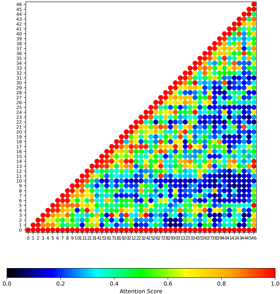
Figure 2: Attention visualization using SAVIS (Seo et al., 2025). Each point represents the attention from the sentence on the x-axis to the sentence on the y-axis when processing the x-axis sentence.
