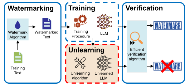
Figure 3: Watermarking as an unlearning metric.
