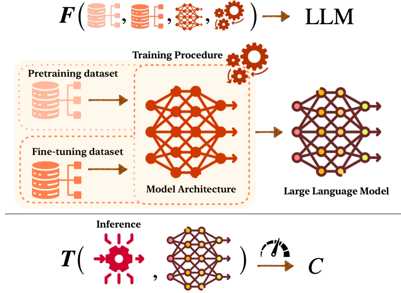
Figure 1: Forward processes in large language models. The forward process generates an LLM from key input ingredients and components: datasets, model architecture, and the training procedure. During inference time, other ingredients such as the prompt examples would affect the desired performance metric C .
