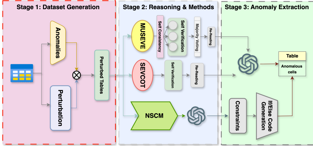
Figure 2: Overview of the methods MUSEVE, SEVCOT, and NSCM.
