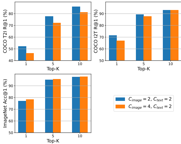
Figure 6: Effects of different expert capacity C .
