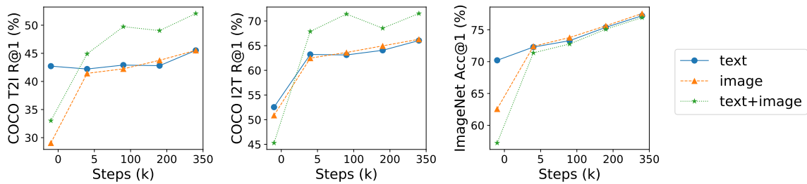
Figure 7: CLIP-UP with MoE upcycling for only the text encoder, image encoder, or both. We observe upcycling both the image and text encoders into MoE generally helps, especially for retrieval tasks.
