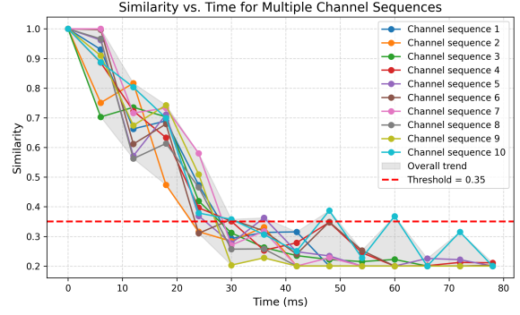
Figure 5: The similarity curve of the channel sequences.
