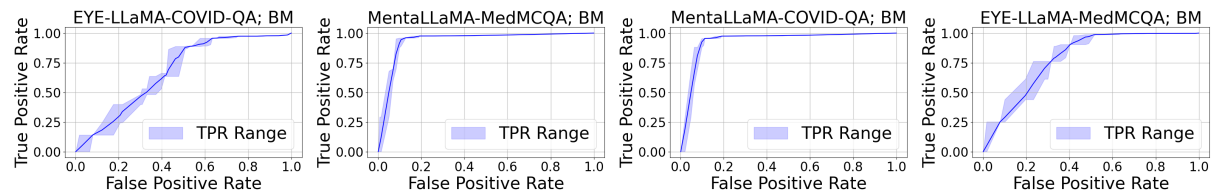
Figure 10: ROC curves with Bonferroni Method as the valid merging function.
