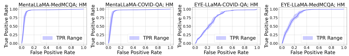
Figure 9: ROC curves with Harmonic Mean as the valid merging function.
