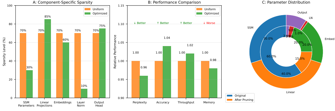
Figure 10: Optimized non-uniform pruning allocation showing component-specific sparsity levels and performance comparisons.
