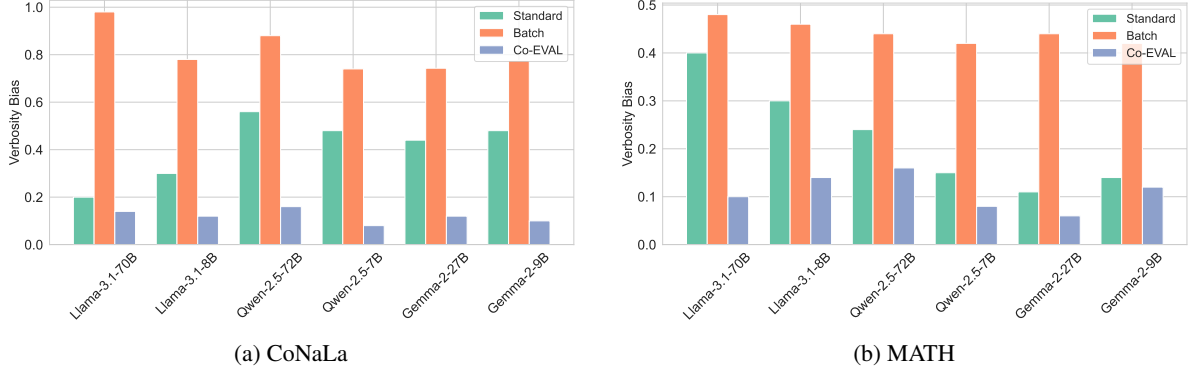
Figure 6: Verbosity bias on CoNaLa and MATH benchmarks. To evaluate verbosity bias, we batch the original responses generated by Llama-3.1-70B-Instruct together with their extended versions that contain intentional errors.
