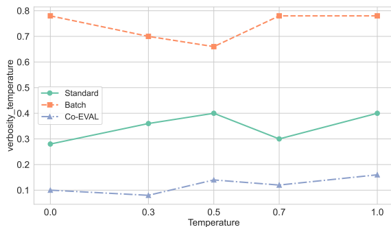
(c) Verbosity
