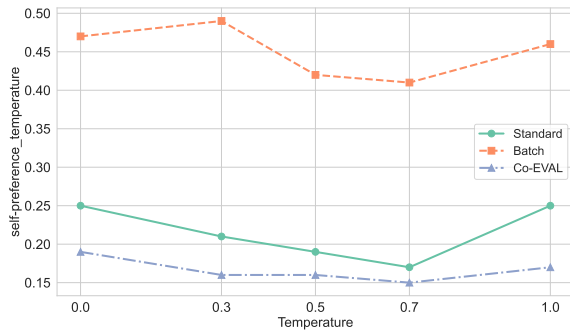
(a) Self-Preference
