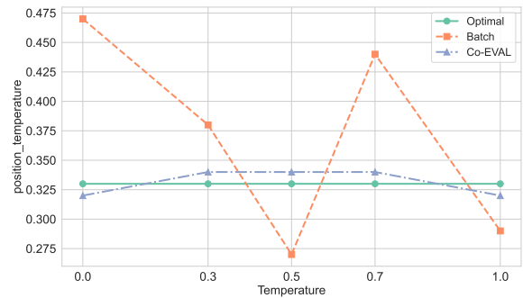
(b) Position
