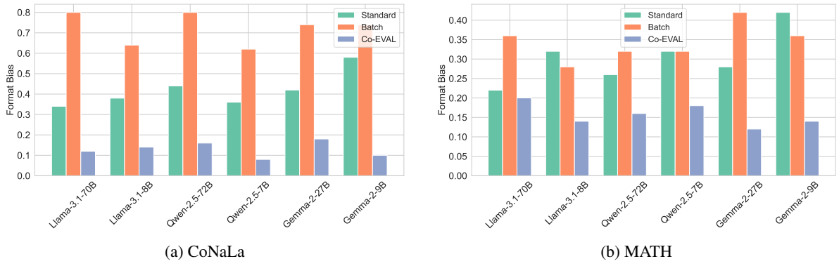
Figure 7: Format bias on CoNaLa and MATH benchmarks. To assess format bias, we batch the original responses generated by Llama-3.1-70B-Instruct together with their formatted counterparts that contain intentional errors.
