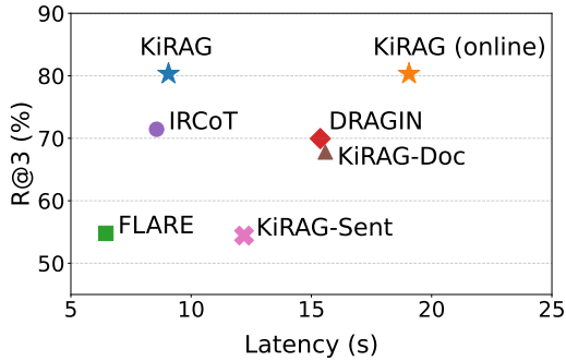
Figure 5: Retrieval performance v.s. average latency per question for different models on the HotPotQA test set. KiRAG (online) represents a variant of our approach where knowledge triples are extracted dynamically during iterative retrieval, without precomputation.
