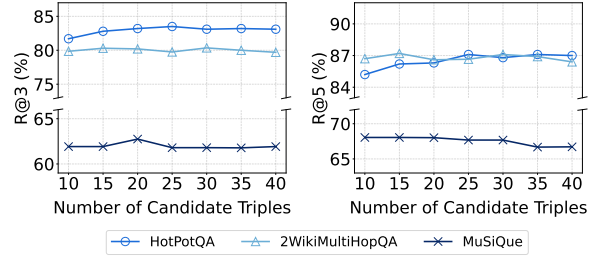
Figure 12: Retrieval performance (%) of KiRAG under different values of N on three multi-hop QA datasets.
