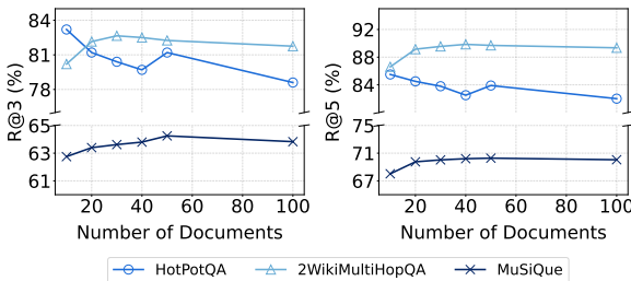
Figure 11: Retrieval performance (%) of KiRAG under different values of K_0 on three multi-hop QA datasets.
