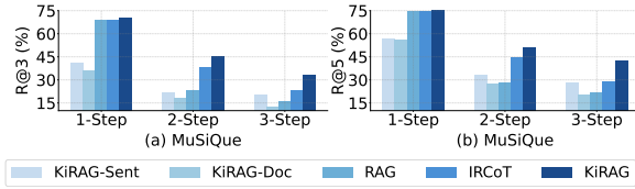
Figure 10: Retrieval performance (%) at different steps on MuSiQue dataset.
