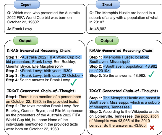
Figure 6: Case study of KiRAG and IRCoT on HotPotQA test set, where the relevant and irrelevant contexts are marked in blue and orange, respectively.
