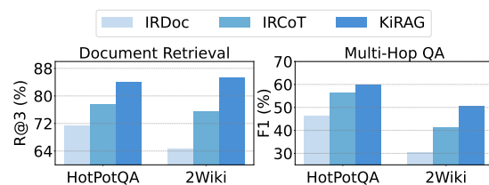
Figure 1: (top) Example of top-ranked documents at each step, with relevant content marked in blue and distracting content in orange. We compare KiRAG with IRCoT (Trivedi et al., 2023) and its variant IRDoc, where we replace generated thoughts with top-ranked documents. (Bottom) The corresponding retrieval and QA performance on HotPotQA and 2Wiki datasets.
