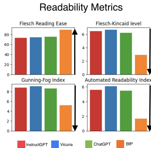
Figure 2: Readability metrics for each model, as well as the Books for Preschoolers human-written dataset (BfP). Note that the direction of the arrow on the side of each chart indicates the direction of improved readability.
