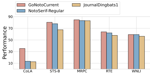
Figure 6: Analysis of fine-tuning on different fonts.
