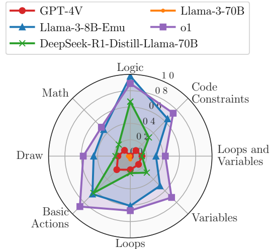
Figure 1: Success rates of different models across different skills in real-world tasks in the XLOGOMINIPROG benchmark.
