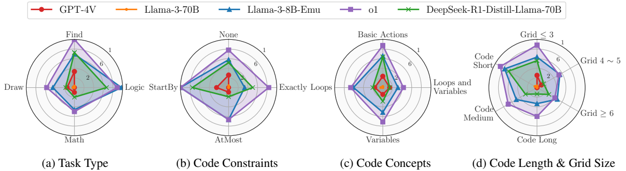
Figure 7: Comparative analysis of models’ capabilities across different dimensions on BASIC. Each chart highlights the models’ capabilities in different aspects within a dimension. Note that code length and grid size are combined in the same chart, as both indicate the difficulty levels of the tasks.
