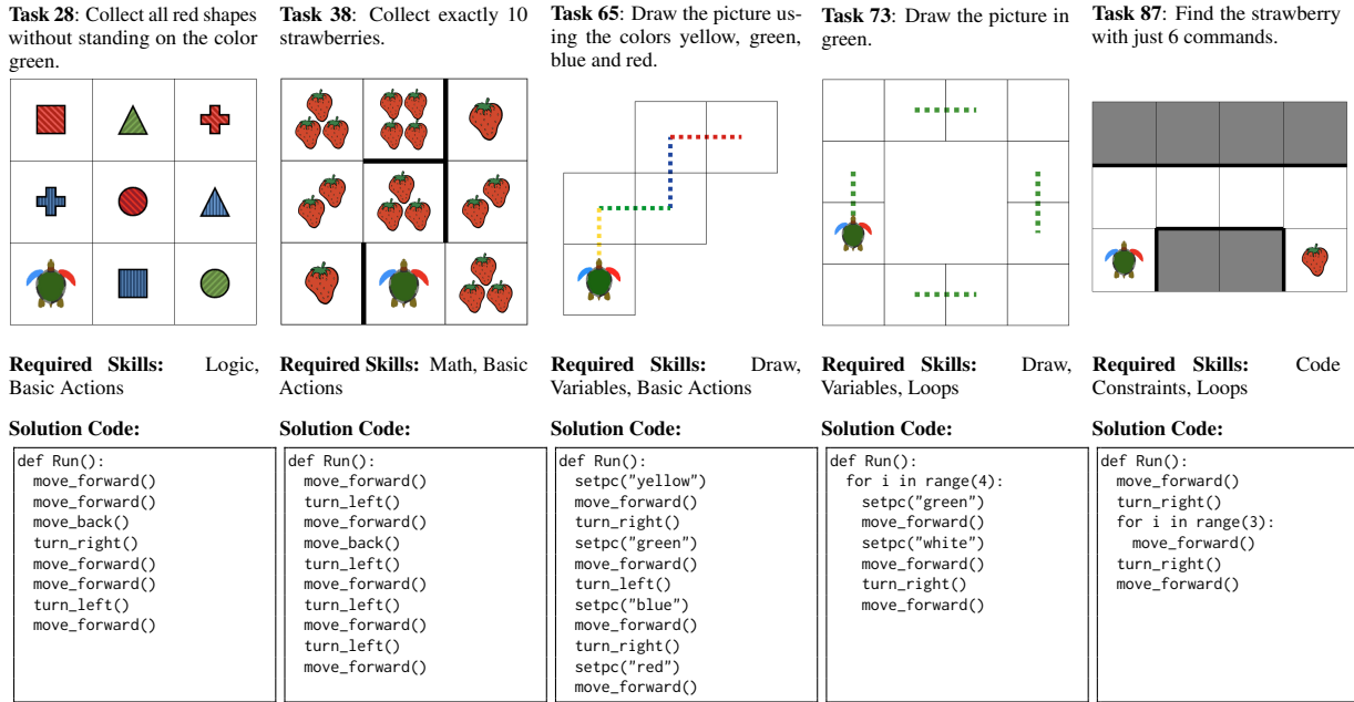
Figure 2: Examples of real-world tasks, required skills, and solution codes in XLogoOnline-Mini.
