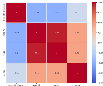
(b) Correlation Heatmap: Tree Edit Distance and CSS IoU with Automated Metrics (Word F1, ROUGE-L).
