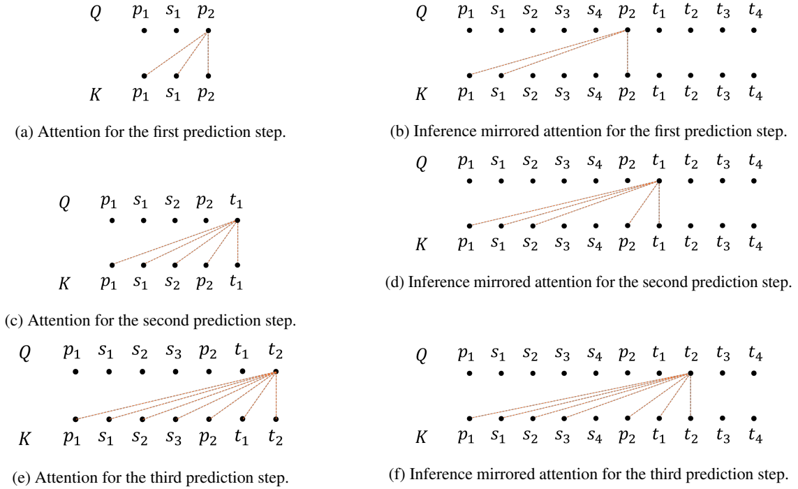
Figure 8: Attention during inference and finetuning for SimulMT.
