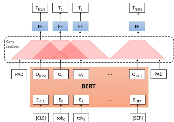
Figure 1: BERT with convolutional model.
