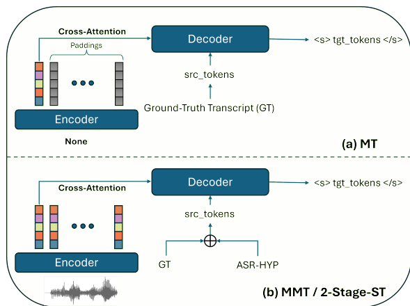
Figure 1: Overview of our approach. ASR-HYP refers to the ASR hypothesis generated. When GT is used, the task is MMT , otherwise it is referred as 2-Stage-ST . The \oplus symbol refers to the XOR operation. Note that special tokens are omitted to simplify illustration.
