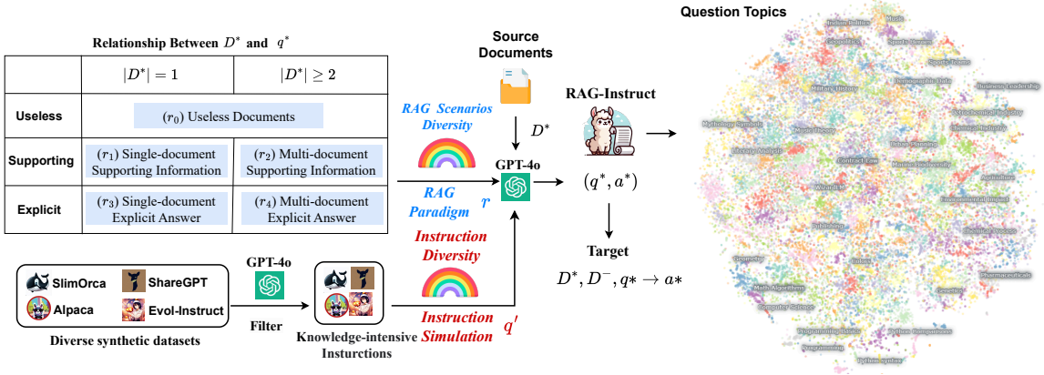
Figure 1: The process of synthesizing data with RAG-Instruct involves ensuring instruction data diversity through five RAG paradigms and Instruction Simulation. The visualization of the question topic is generated using Atlas.
