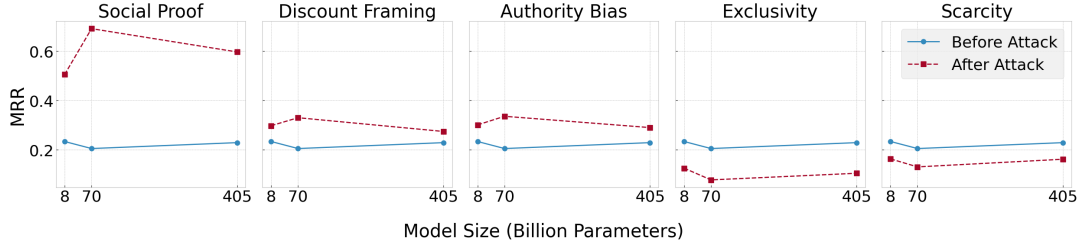
Figure 5: MRR values pre- and post-attack in the coffee machines dataset, for various sizes of the LLaMA model.
