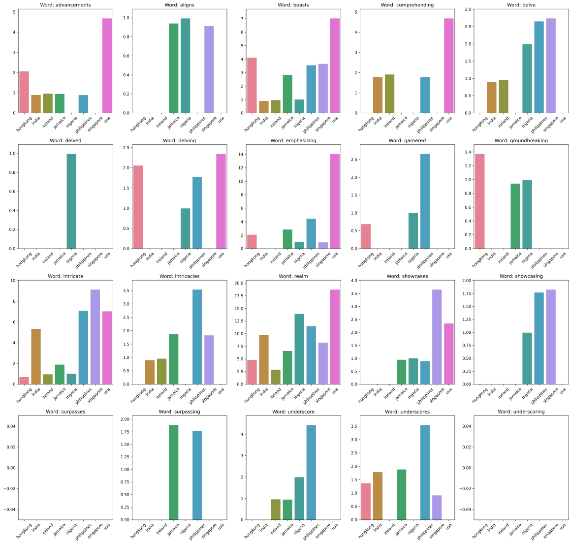
Figure 8: Word frequencies for selected lexical items across various English variants.
