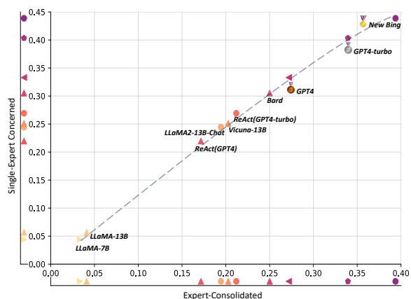
Figure 4: Performance difference on the experts-consolidated and single-expert-focused set.
