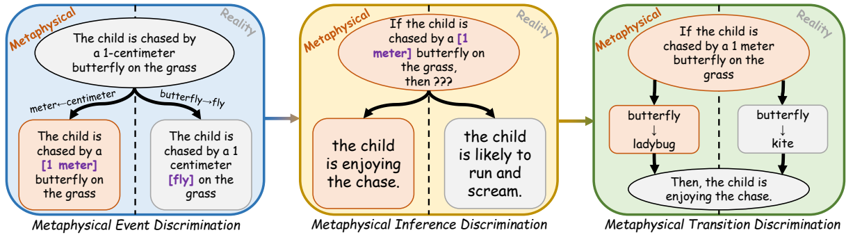
Figure 2: The three steps in metaphysical reasoning. Our motivation behind this is that, by conquering all steps sequentially, a conscious agent could answer: (1) Will the change occur in reality? (2) What will the change cause? (3) What change can make a metaphysical (desired) inference plausible?
