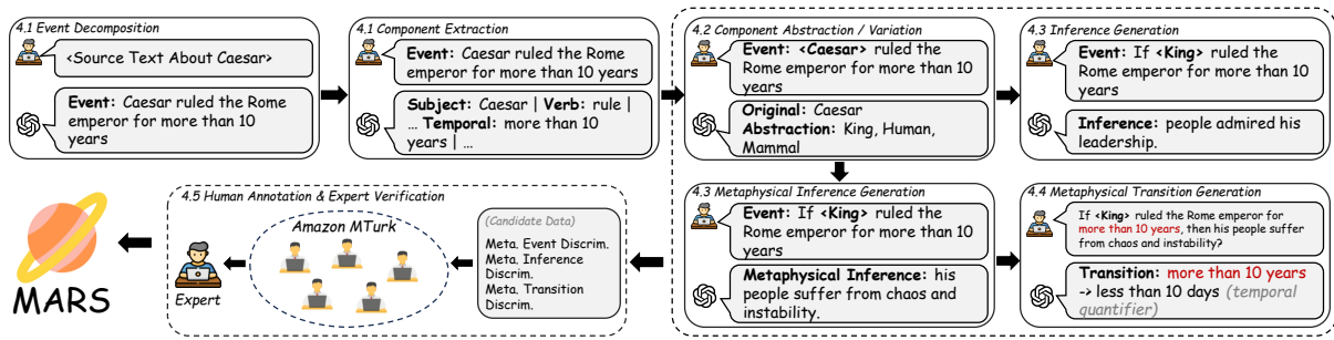
Figure 5: An overview of our benchmark curation pipeline with running examples.
