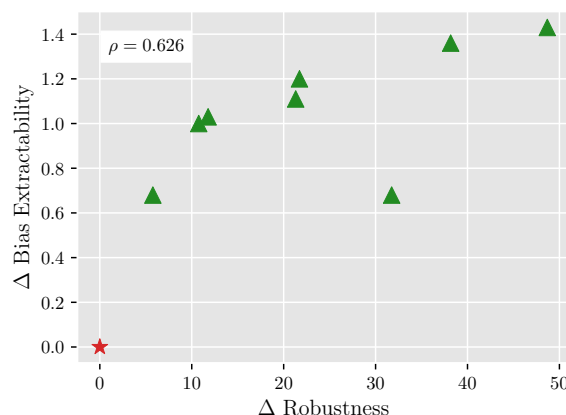
Figure 1: Amount of subsequence bias extracted from different language models vs. the robustness of models to the bias. Robustness is measured as improvement of the model on out-of-distribution examples, while extractability is measured as the improvement of the probe’s ability to extract the bias from a debiased model, compared to the baseline.
