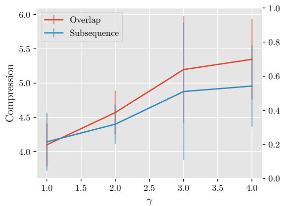
Figure 2: Compression of a DFL model with an implicit bias model on Overlap/Subsequence probing tasks vs. the focusing parameter \gamma , for MNLI. As \gamma increases, the bias becomes more extractable.
