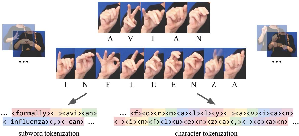
Figure 1: Visual depiction of subword- vs. character-level tokenization as it relates to sign language translation. Color highlights are a visual aid for token boundaries. We omit faces in the figure for privacy. Fingerspelled spans such as “avian influenza” within larger sentences must be mapped to sequences like <avi><an><influenza><, >< can> in the T5 subword vocabulary; the model can only know how these tokens are spelled through fingerspelling data coverage (less likely) or from text pretraining (more likely). Character-level tokenization makes the mapping much more straightforward, at the expense of increasing sequence length for the rest of the sentence.
