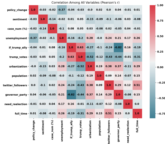
Figure 4: Correlation across all variables.
