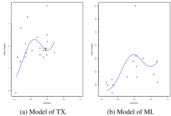
Figure 5: Causal models by continuous-valued propensity score matching of TX and MI.
