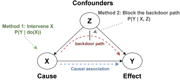
Figure 2: Backdoor Adjustment.
