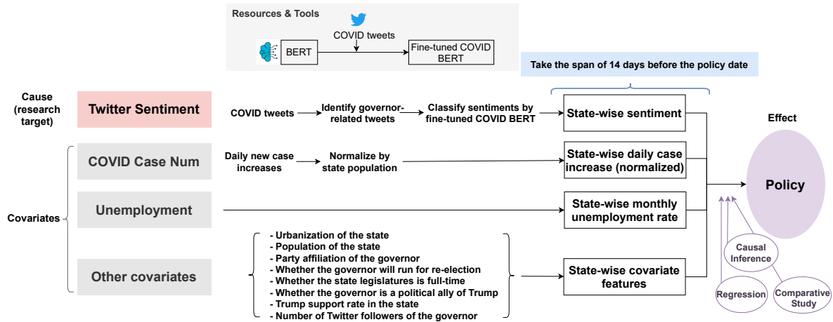
Figure 1: The data collection pipeline and architecture of our system to predict the state-wise COVID policies.
