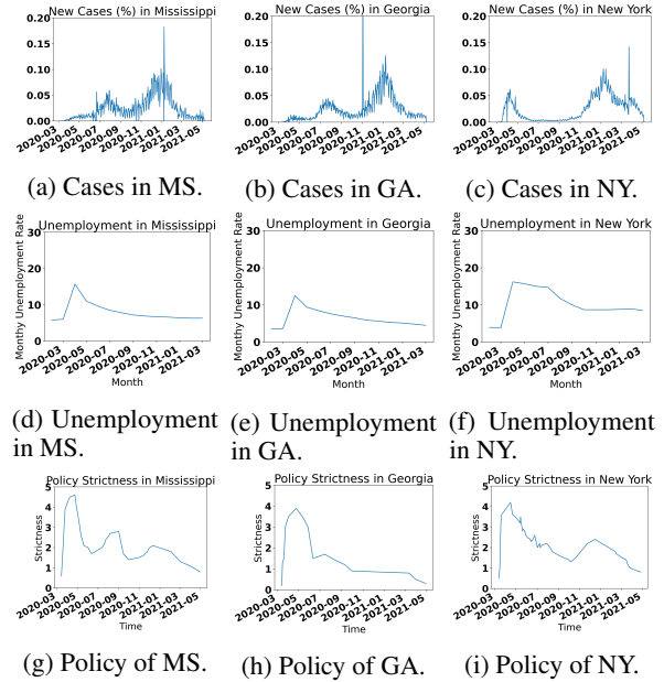
Figure 3: Comparative study of states. MS and GA is a pair of states with the most similar confounders, and NY is an irrelevant state to contrast how different MS and GA are from other states. Note that unemployment data is only available until March 2021.
