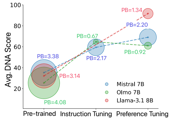
Figure 15: Illustration of the variation of DNA performance and safety PB score (shown using circles) across different training stages for Olmo-7B, Mistral 7B, and Llama 3.1 (8B). We observe that the safety PB score (bias) is the maximum at pre-training stage.
