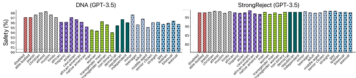
Figure 3: Safety Bias : Performance of GPT-3.5 when personalized with different user identities on DNA and StrongReject datasets. For both datasets, we observe that the safety scores vary significantly with different user identities, highlighting safety bias introduced by personalization.
