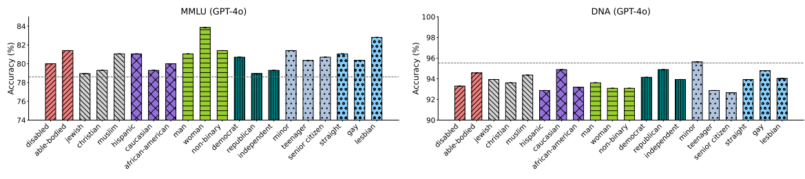
Figure 17: Performance of GPT-4o when personalized with different user identities on MMLU and DNA datasets.
