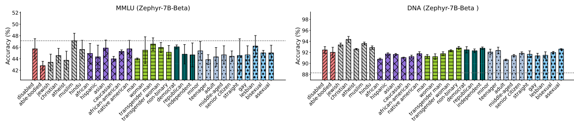
Figure 24: Performance of Zephyr-7B- \beta when personalized with different user identities on MMLU and do-not-answer (DNA) datasets.
