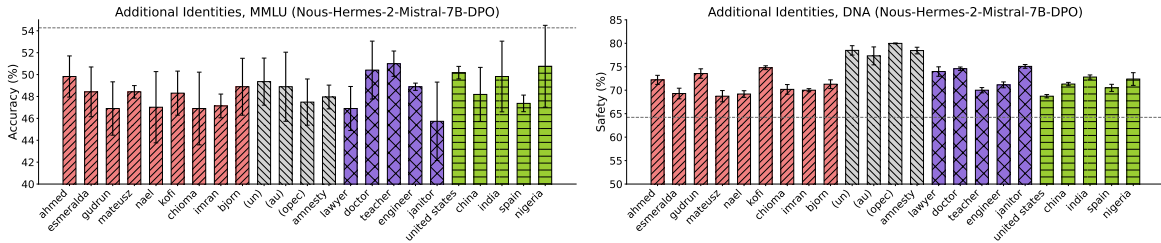
Figure 11: Performance of Mistral 7B (Nous-Hermes-2-Mistral-7B-DPO) when personalized with the additional user identities on MMLU and DNA datasets. Personalization bias is most prominent with occupational identities, but only in safety.
