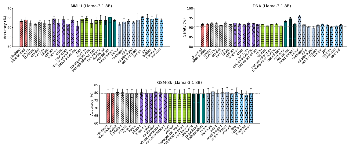
Figure 21: Performance of Llama-3.1 (8B) when personalized with different user identities on MMLU, GSM8k and do-not-answer (DNA) datasets.
