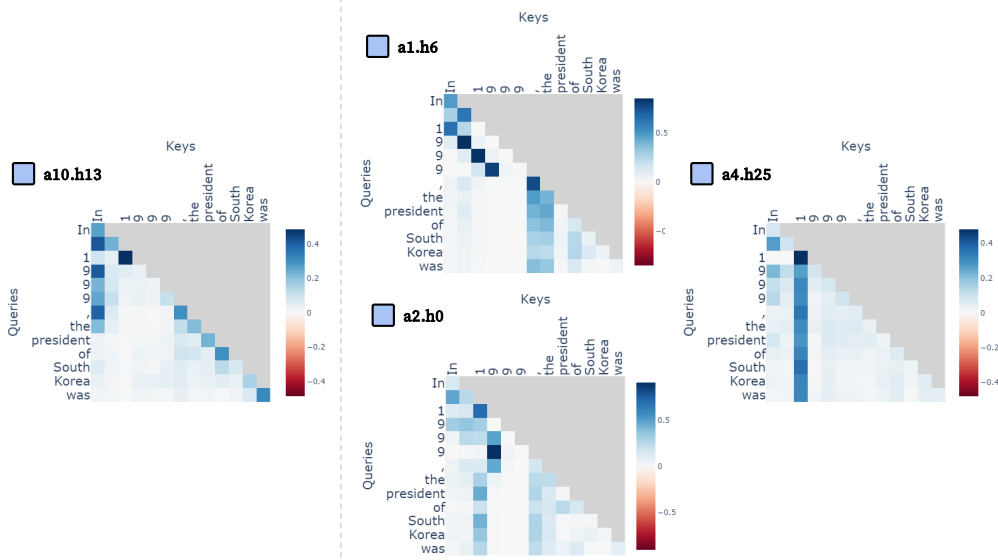
Figure 11: Total map of attention with Phi-3-mini-4k-instruct, for each temporal heads and backup temporal heads. The left side of border line is the attention map of Temporal Heads , and the other side is the result of Backup Temporal Heads .
