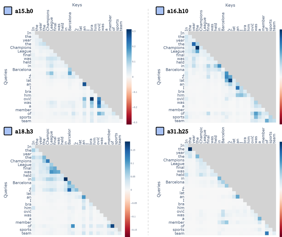
Figure 14: Temporal knowledge circuit from textual temporal conditioned prompt. Here, we change the temporal condition "In 1999" into "In the year the Champions League final was held in Barcelona", which model already correctly recalls the answer Malmö FF . The temporal knowledge circuit successfully catches temporal conditioning even with alias based on event based textual conditioning, with correctly showing off temporal knowledge heads and some backup temporal heads. Figure of downside is the attention maps for each temporal heads and backup temporal heads. Each of those figures highlight various tokens in conditioning part of prompt.
