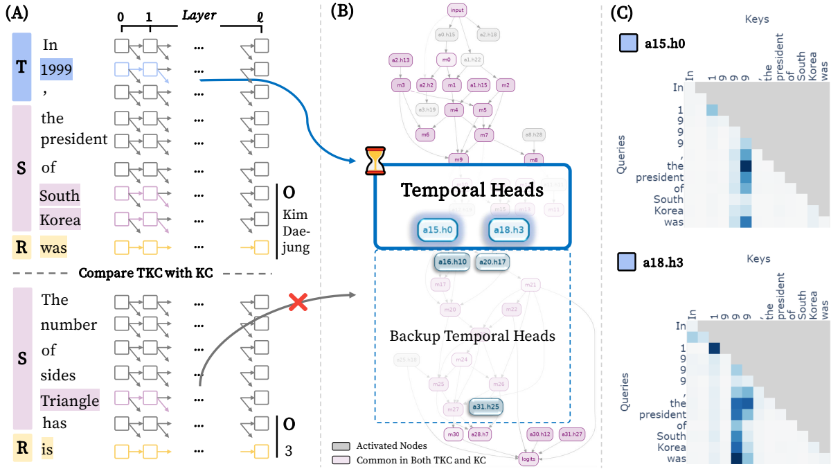
Figure 2: Overview of temporal knowledge circuit analysis. (A): Construct temporal knowledge circuits (TKCs), and compare it with general knowledge circuits (KCs) using time-invariant knowledge. Circuits reproduce residual streams for time T , subject S and relation R . This verifies temporal heads only found in each different TKCs of various year T_k . (B): Example of simplified TKC. Here, basic knowledge nodes is colored violet, (common in both), while Temporal Heads is highlighted. (C): Attention map for Temporal Heads. a15.h0 means the 15th layer’s first attention head. Each head’s attention pattern is visualized with the attention weight assigned by the queries (row) to the keys (column). Queries are the tokens distributing attention, and Keys are the tokens receiving attention. Values represent attention weights, indicating the strength of this focus. Total results are in Figures 7–11.
