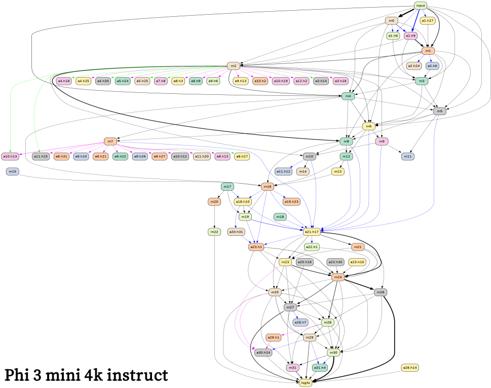
Figure 8: Temporal knowledge circuit of Qwen 1.5 and Phi 3 mini. Those are simplified version of total circuit according to each nodes and edges' importance of using same \tau = 0.1 as threshold.
