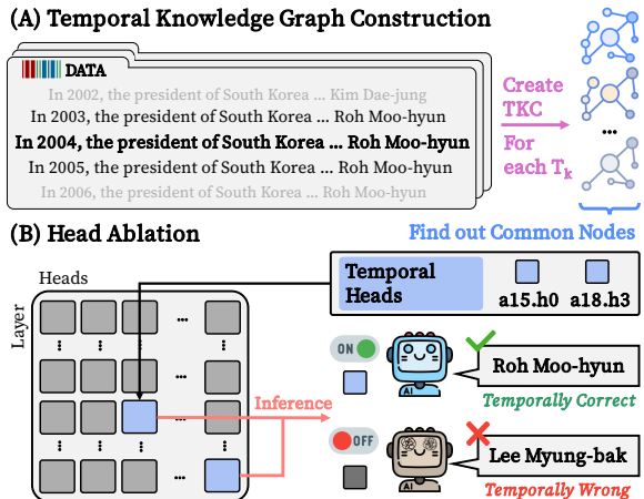
Figure 1: Temporal Heads exist within various TKCs at different times T_k . Ablating them disrupts the model’s temporal alignment, yielding incorrect objects.
