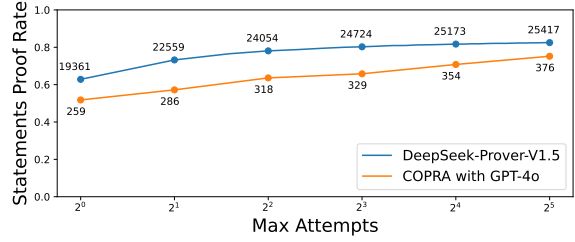
Figure 6: The proof rates of two SOTA theorem provers on FormalStep . The numbers indicate the total quantity of statements that have been successfully proved. Note that COPRA is significantly more resource-intensive due to its reliance on GPT-4o; therefore, it is tested on a randomly selected subset of 500 statements, while DeepSeek-Prover-V1.5 is evaluated on full FormalStep , comprising a total of 30,809 statements.
