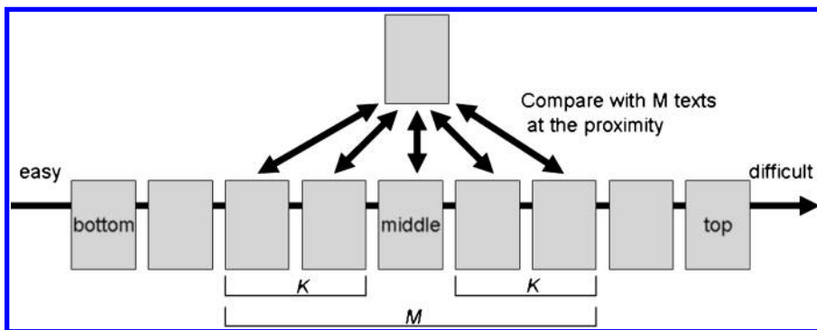
Figure 3 Robust comparison.
