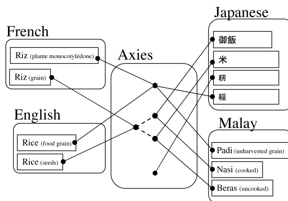
Figure 2. Illustration of Papillon's macrostructure.
