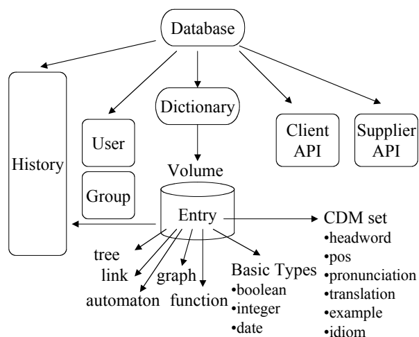
Figure 1. The DML Framework
