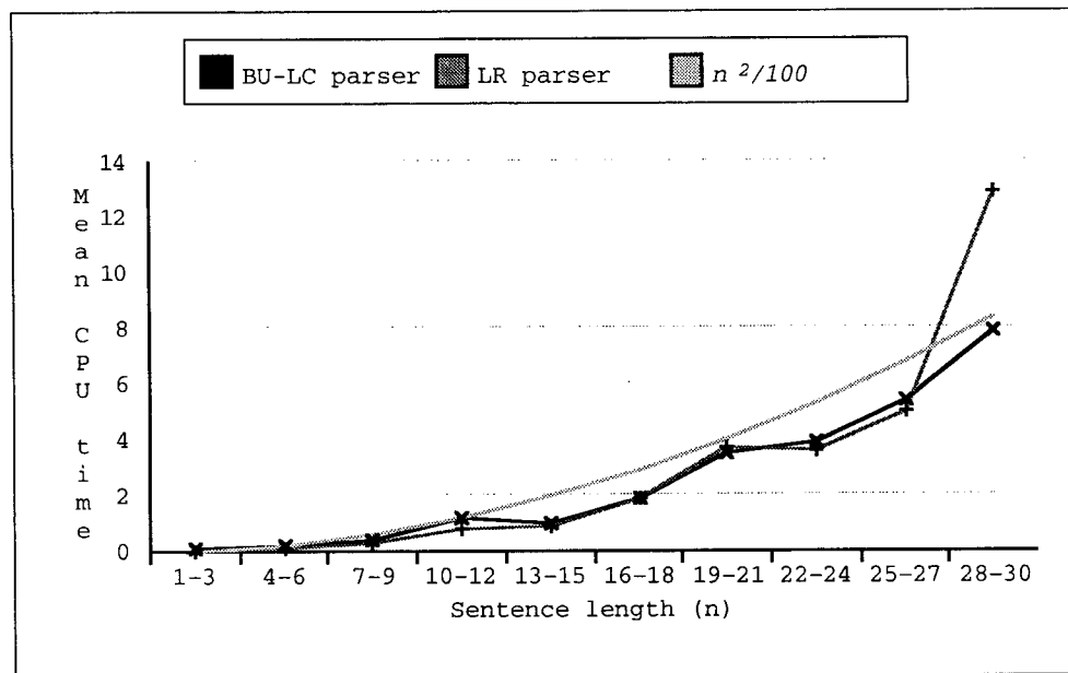
Figure 1: Mean parse times (in CPU seconds on an HP9000/710 workstation) for the test sentences with the BU-LC and LR parsers. A quadratic function is also displayed.
