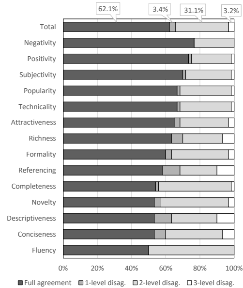
Figure 2: Annotators agreement.
