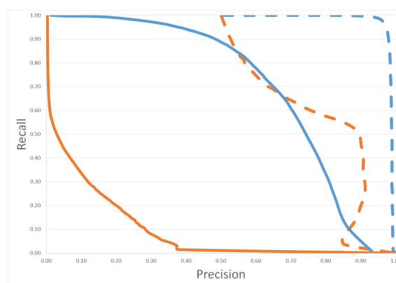
Figure 3: Precision-recall curves for our compound classifier for two languages: German (red) and Finnish (blue). Unbalanced test set results are shown with solid lines. Balanced test set results are shown with dashed lines.
