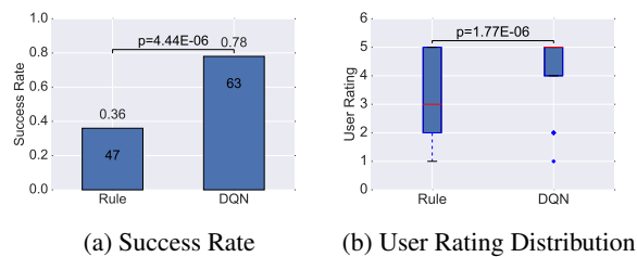
Figure 6: Performance of the rule-based agent versus DQN agent tested with real users: (a) success rate, number of tested dialogues and p-values are indicated on each bar; (b) Distribution of user ratings for two agents (difference in mean is significant with p < 0.01 ).
