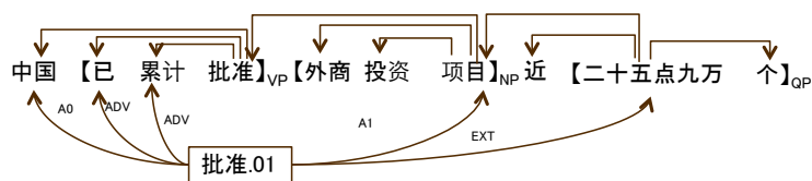
(b) Wrong SRL result brought by MALT parse errors
