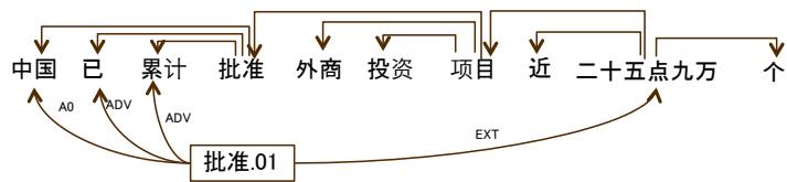
(b) Wrong SRL result brought by MALT parse errors
