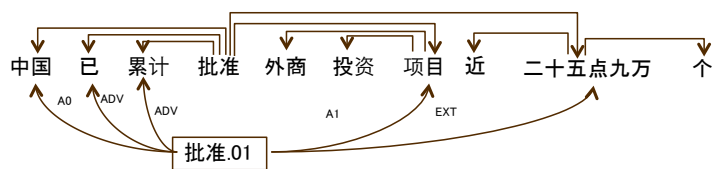
(a) Gold SRL result with gold dependency tree
