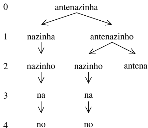
Figure 1: Lemmatization of antenzinha
