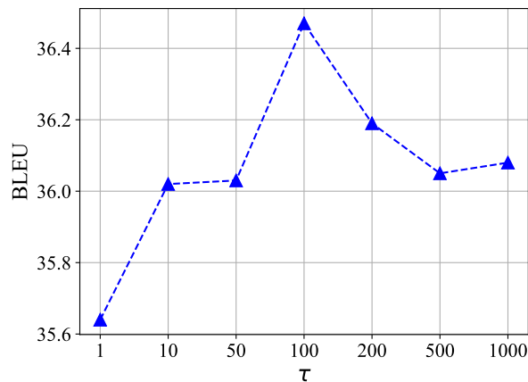
Figure 3: BLEU scores with different \tau and fixed k ( k = 64 ) on the validation set of IWSLT’14 De-En dataset.
