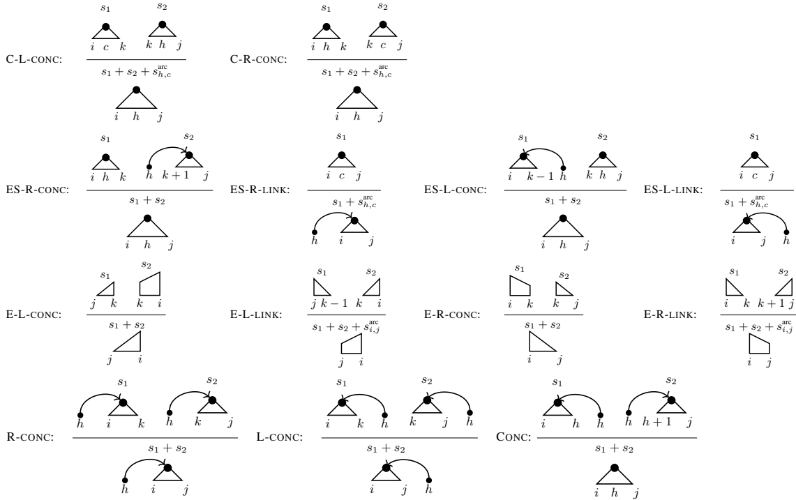
Figure 3: Deductive rules of the parsing algorithms of Collins (1996) (the first line), Eisner and Satta (1999) (the second line), Eisner (1997) (the third line). The last line is the resulting deduction rules after applying head-splitting on ES-L-CONC and ES-R-CONC. All deduction items are annotated with their scores. We only consider the pure dependency versions of these algorithms. We omit axiom items for simplicity.
