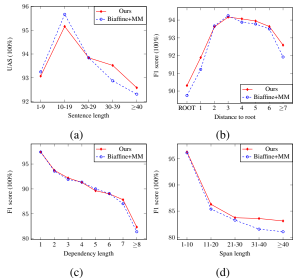
Figure 4: Error analysis on the CTB test set.
