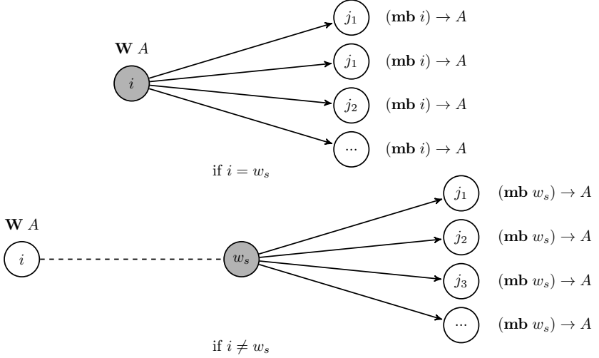
FIGURE 6 Possible Worlds Hierarchy of \llbracket \textit{would} \rrbracket_{M\text{-}TTDLA}
