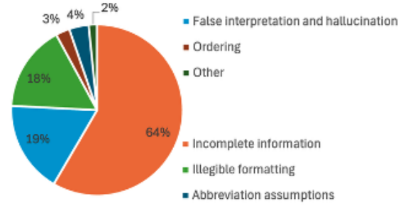
Figure 3: Reasons for incorrect NLRs based on human assessment of model-produced NLRs.
