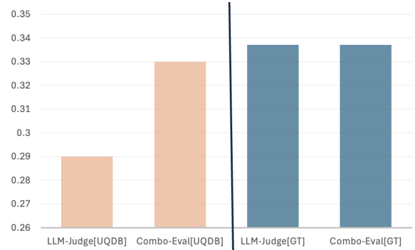
Figure 12: Percentage reduction in incorrect NLR judgments for LLM-judge and Combo-Eval methods compared to Metrics-based evaluation method in UQDB (left) and GT (right) scenarios.
