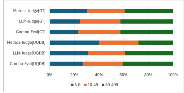
Figure 5: Breakdown of incorrect judgments by result size across evaluation methods (Metrics-based, LLM-judge, and Combo-Eval) for GT and UQDB scenarios, showing higher misjudgments by LLM-as-a-judge on higher result sizes.
