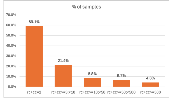
Figure 7: Result size distribution in the BIRD-dev dataset. rc=row count; cc=column count.
